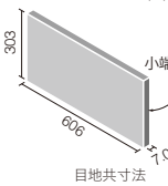
ECP-6301T/*(R)
