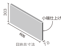
ECP-6301T/**(R)
